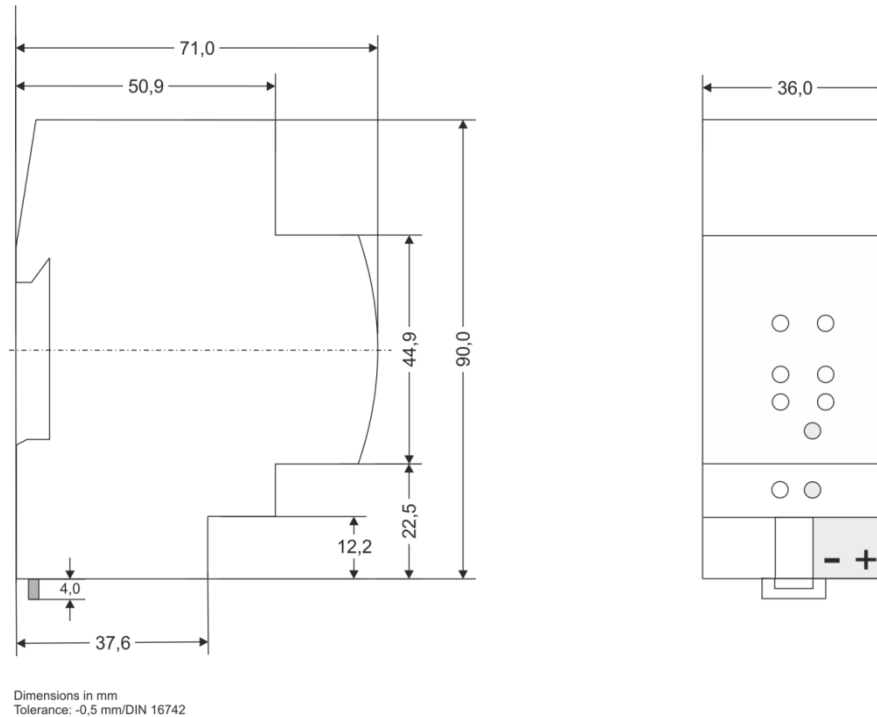
Figure 19: Dimension drawings
