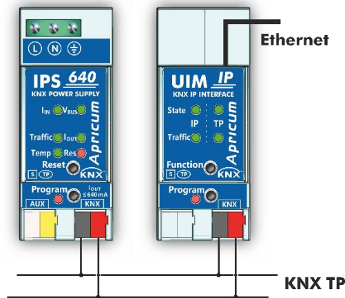
Figure 2: Connection Scheme
